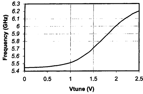
Fig. 6 Measured tuning characteristic of the VCO
