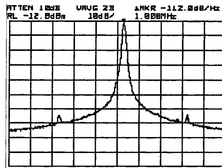
Fig. 5 Spectrum of the VCO at 5.8 GHz observed in HP 8563E
